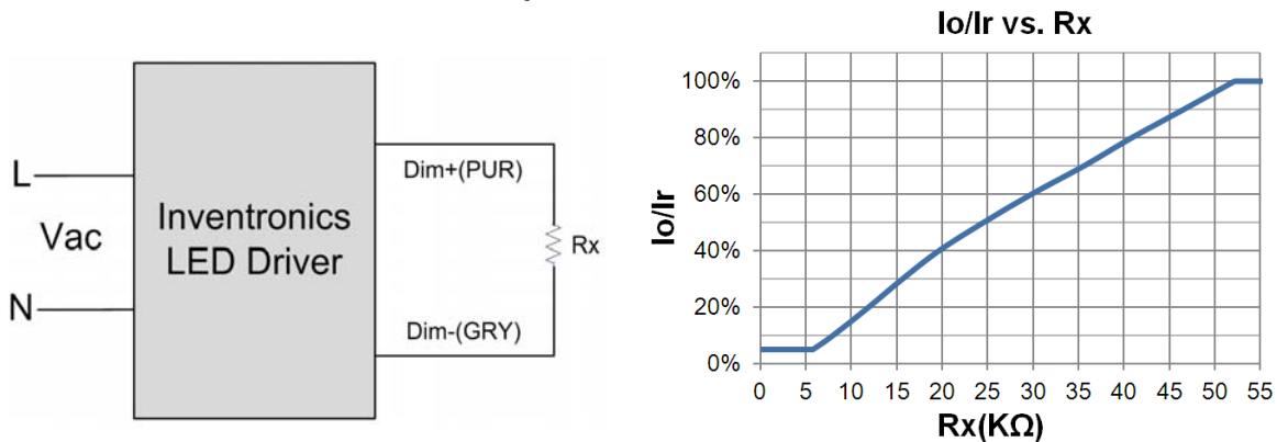
Implementation 2: External Resistor
