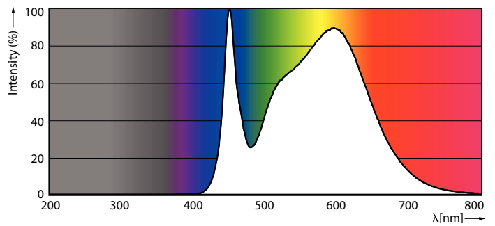
Spectral Power Distribution Colour - 115CC/LED/840/LS EX39 G2 BB 277-480V 3/1
