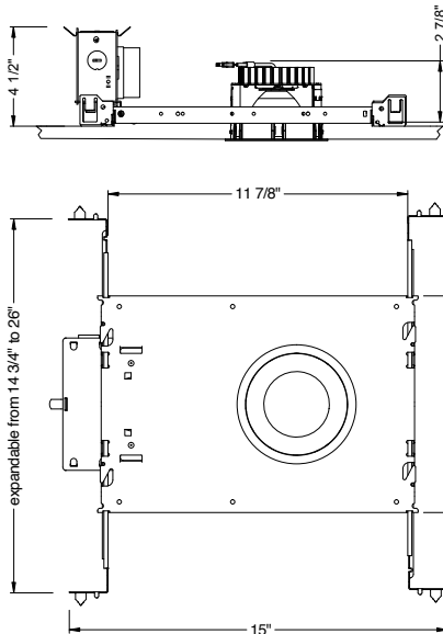
ceiling cutout 4 3/8" diameter
