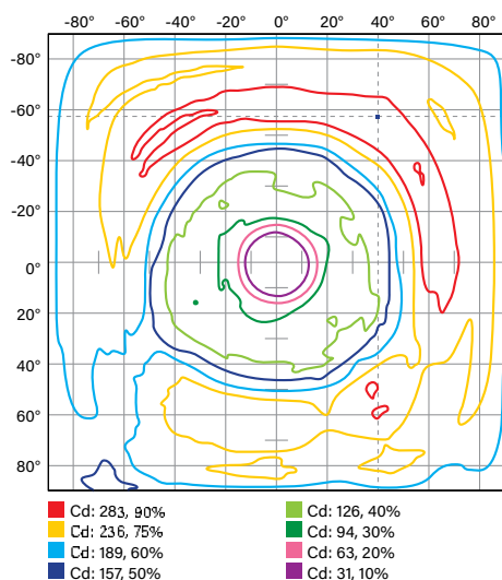
ISOCANDELA PLOT
