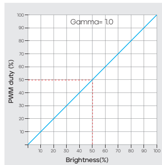
Dimming curve
