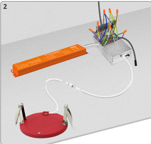
2. Connect wires as shown on electrical diagram.
