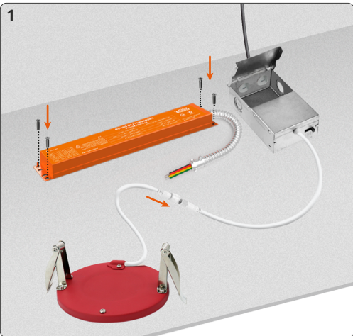
1. Secure the battery back-up to the ceiling.
