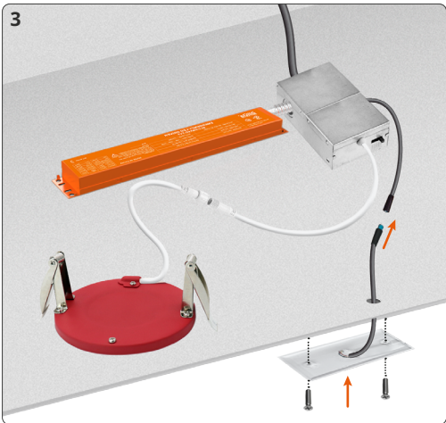
3. Connect test switch and secure it in the hole on surface.
