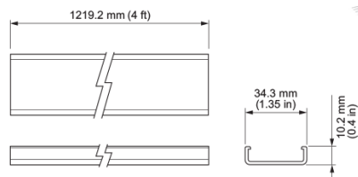
Mounting Track
