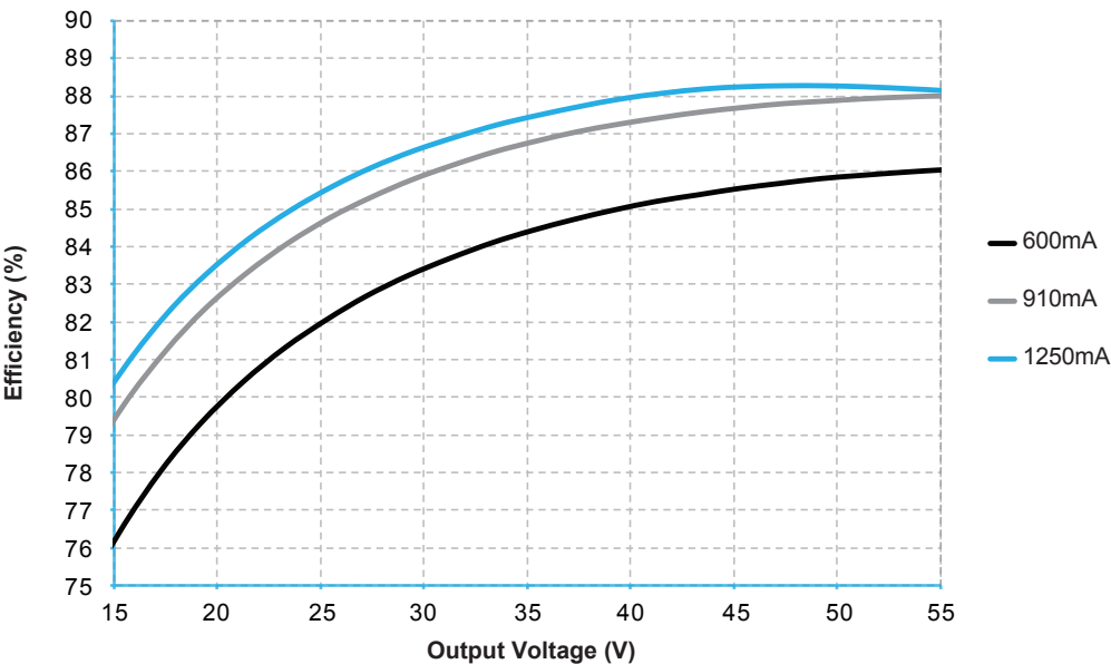
Efficiency @ 120V
