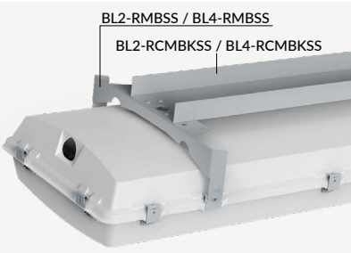
BL2 & BL4-RCMBKSS Stainless Steel Rigid Center Mounting Plate for single point mounting. Requires use of HUB 3/4 and RMBSS.
