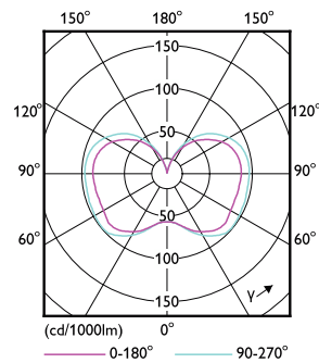
Light Distribution Diagram - 36-27-18CC/LED/3PW/3CCT/E26 BB 6/1
