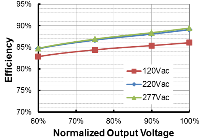
EUG-192D400DT( I_o=4000mA ) Efficiency vs. Output Voltage
