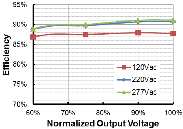
EUG-192D400DT( I_o=2650mA ) Efficiency vs. Output Voltage
