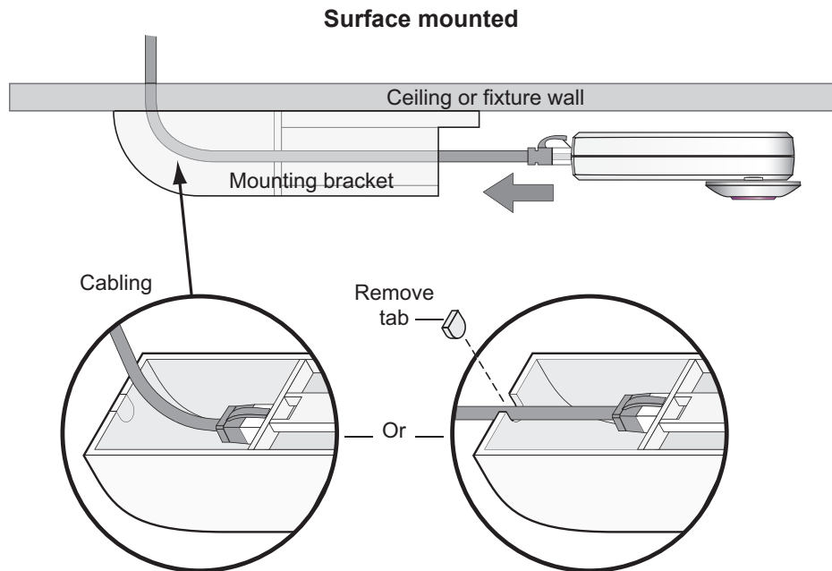
Surface Mount using LMLS-MB2 Mounting Bracket
