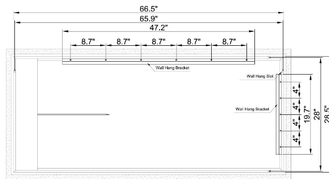
REAR VIEW
