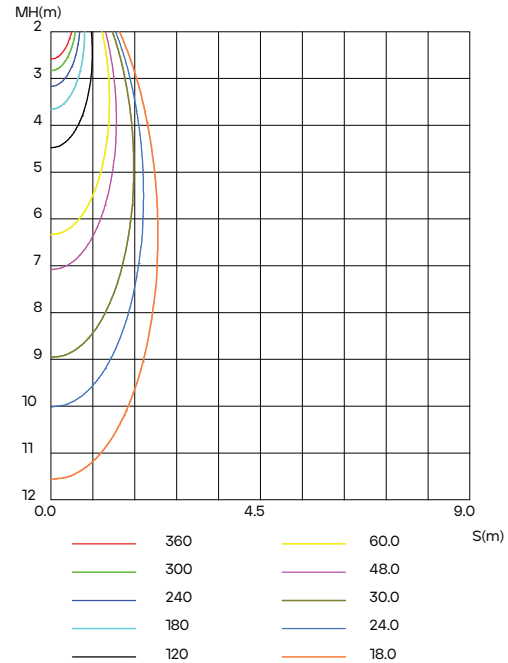
C0 PLANE ISOLUX DIAGRAM (UNIT:lx/klm)
