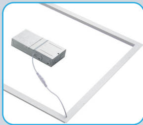
DRIVER WITH CCT & WATTAGE SELECT SWITCH
