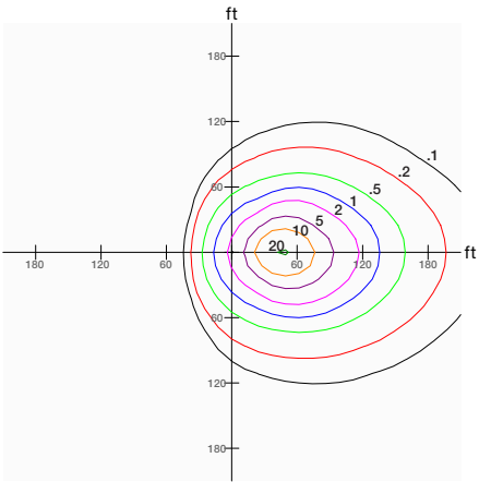
600W Fixture, 4x4 Distribution, Tilted 45°, Mounted at 60'
