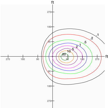
1500W Fixture, 4x4 Distribution, Tilted 45°, Mounted at 90'
