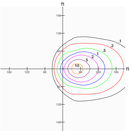
500W Fixture, 5x5 Distribution, Tilted 45°, Mounted at 60'
