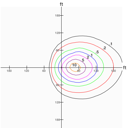
400W Fixture, 4x4 Distribution, Tilted 45°, Mounted at 60'
