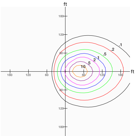
500W Fixture, 4x4 Distribution, Tilted 45°, Mounted at 60'
