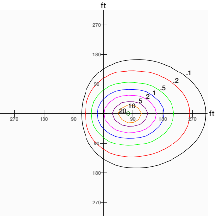
1000W Fixture, 3x3 Distribution, Tilted 45°, Mounted at 90'
