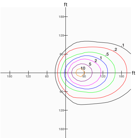
400W Fixture, 5x5 Distribution, Tilted 45°, Mounted at 60'
