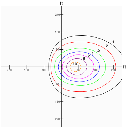
1000W Fixture, 4x4 Distribution, Tilted 45°, Mounted at 90'
