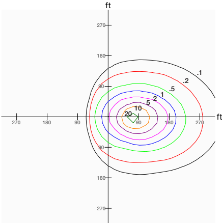
1200W Fixture, 4x4 Distribution, Tilted 45°, Mounted at 90'
