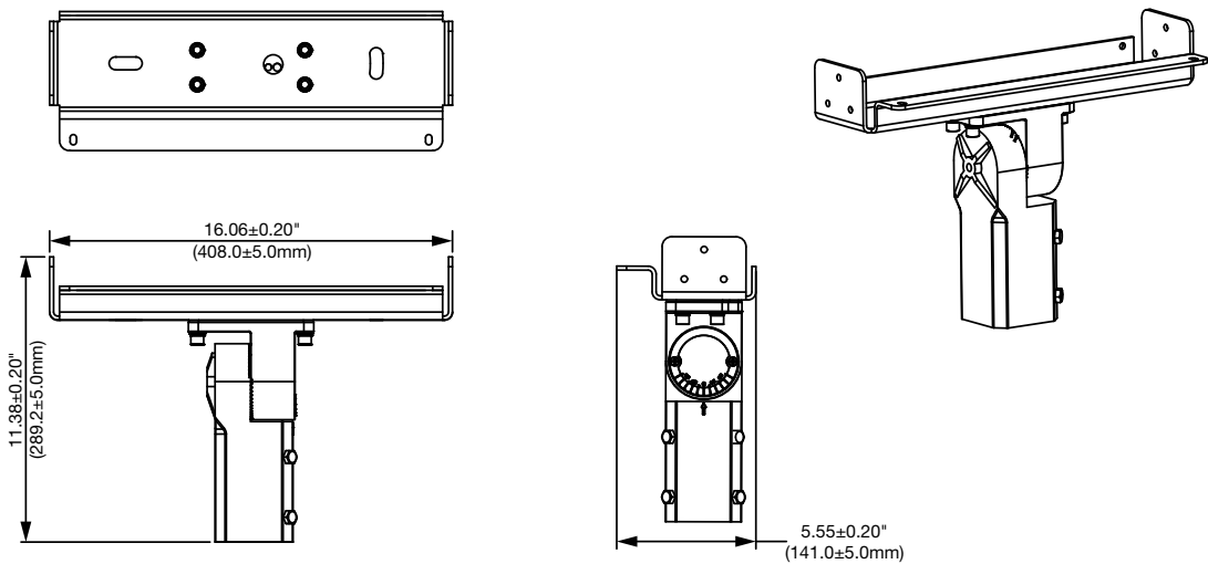
SLIP FITTER 400-600W
