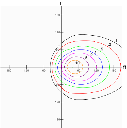
600W Fixture, 5x5 Distribution, Tilted 45°, Mounted at 60'
