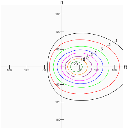
750W Fixture, 4x4 Distribution, Tilted 45°, Mounted at 60'
