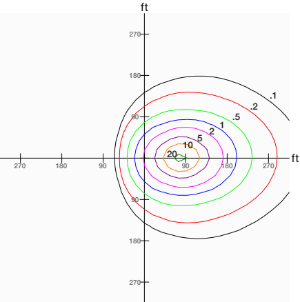
1200W Fixture, 3x3 Distribution, Tilted 45°, Mounted at 90'
