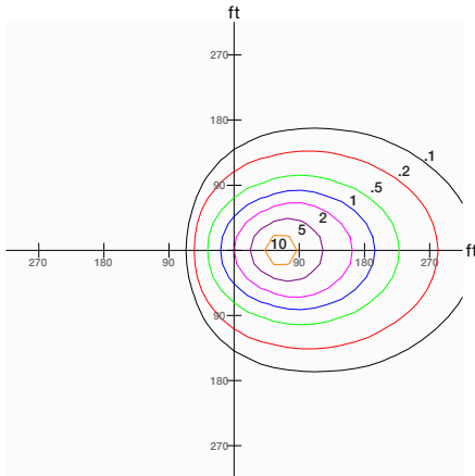
1000W Fixture, 5x5 Distribution, Tilted 45°, Mounted at 90'
