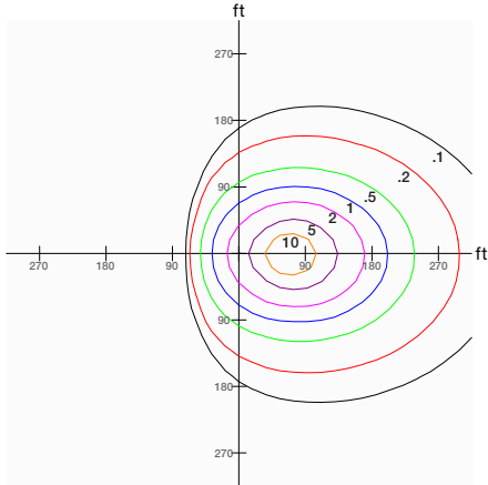
1500W Fixture, 5x5 Distribution, Tilted 45°, Mounted at 90'
