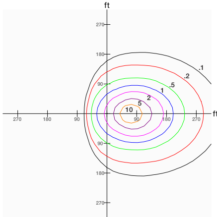
1200W Fixture, 5x5 Distribution, Tilted 45°, Mounted at 90'
