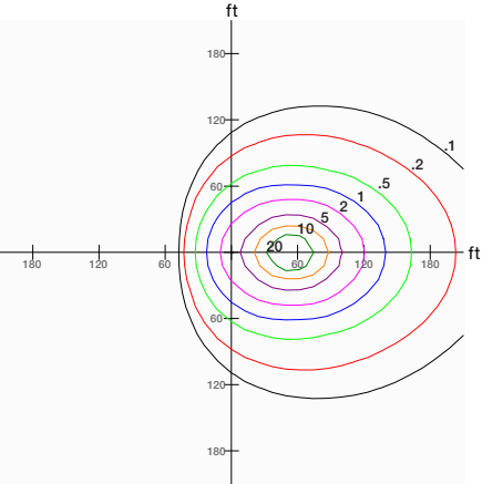
750W Fixture, 3x3 Distribution, Tilted 45°, Mounted at 60'
