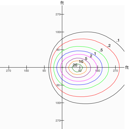
1500W Fixture, 3x3 Distribution, Tilted 45°, Mounted at 90'
