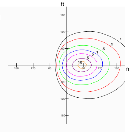
500W Fixture, 3x3 Distribution, Tilted 45°, Mounted at 60'
