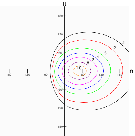
600W Fixture, 3x3 Distribution, Tilted 45°, Mounted at 60'
