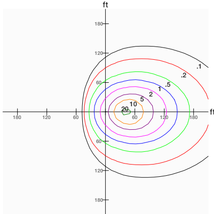
750W Fixture, 5x5 Distribution, Tilted 45°, Mounted at 60'
