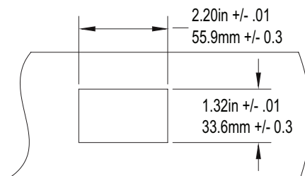
Figure 8. Cutout Dimensions for LMFC-2RJ
