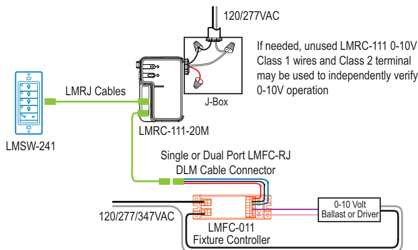
Figure 9. Connecting LMKT-OEM1 Test Kit devices to Device Under Test (DUT)
