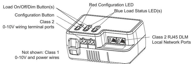
Figure 10. LMRC-112 Detail
