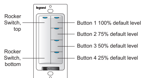
Figure 11. LMSW-105 Detail
