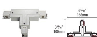
PRO-M436R-BK PRO-M436R-WH 3-Circuit reversing 'T' connector. Right turn.
