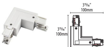
PRO-0435L-BK PRO-0435L-WH Left turn 3-circuit connector. To connect two track sections at a right angle. Ground inside turn.
