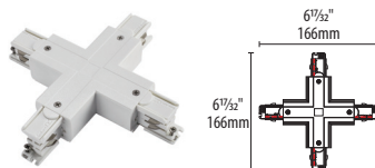
PRO-0437-BK PRO-0437-WH 3-Circuit 'X' connector. To connect four track sections into a cross configuration.
