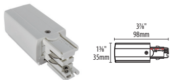
PRO-0431R-BK PRO-0431R-WH 3-Circuit live-end connector. Ground on right. 3-circuit track compatible.
