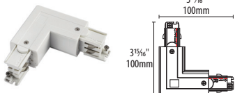
PRO-0435R-BK PRO-0435R-WH Right turn 3-circuit connector. To connect two track sections at a right angle. Ground outside turn.
