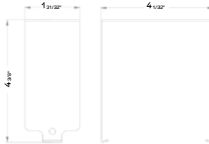
Surface Mount for CLHB-3 CLHB-4
