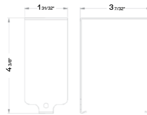
Surface Mount for CLHB-1, CLHB-2
