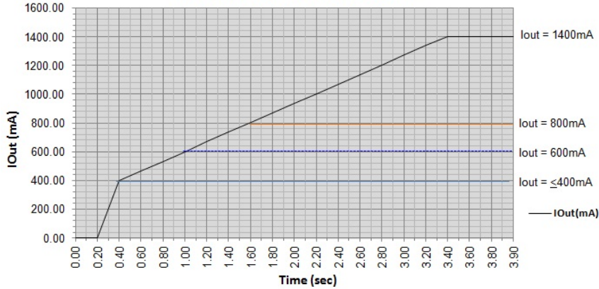
Example Startup Times vs Output Current
