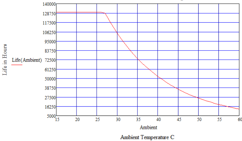
LP40W Estimated Life Full Load @ 120Vac
