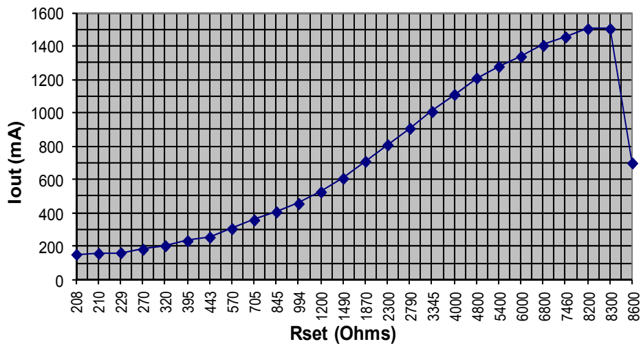
Output Current (mA) vs. Rset (Ohms)
