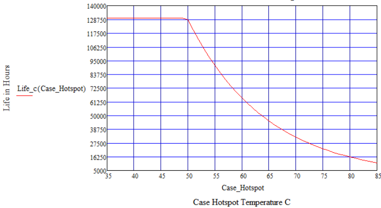
LP40W Estimated Life Full Load @ 120Vac
