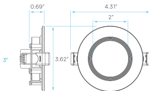
CUTOUT: Ø 3"
