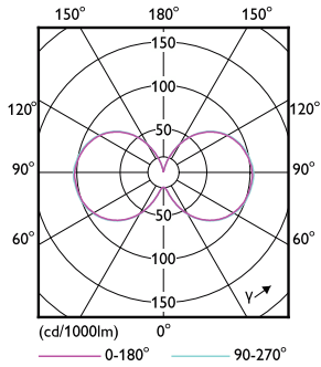
Light Distribution Diagram - 145CC/LED/3CCT/LS EX39 BB 3/1
