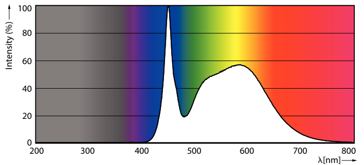
Spectral Power Distribution Colour - 145CC/LED/3CCT/LS EX39 BB 3/1
