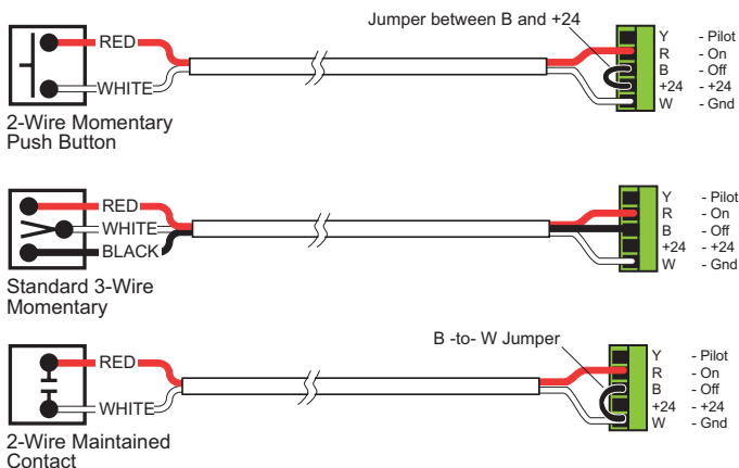
Fig.5: Low Voltage Switches
