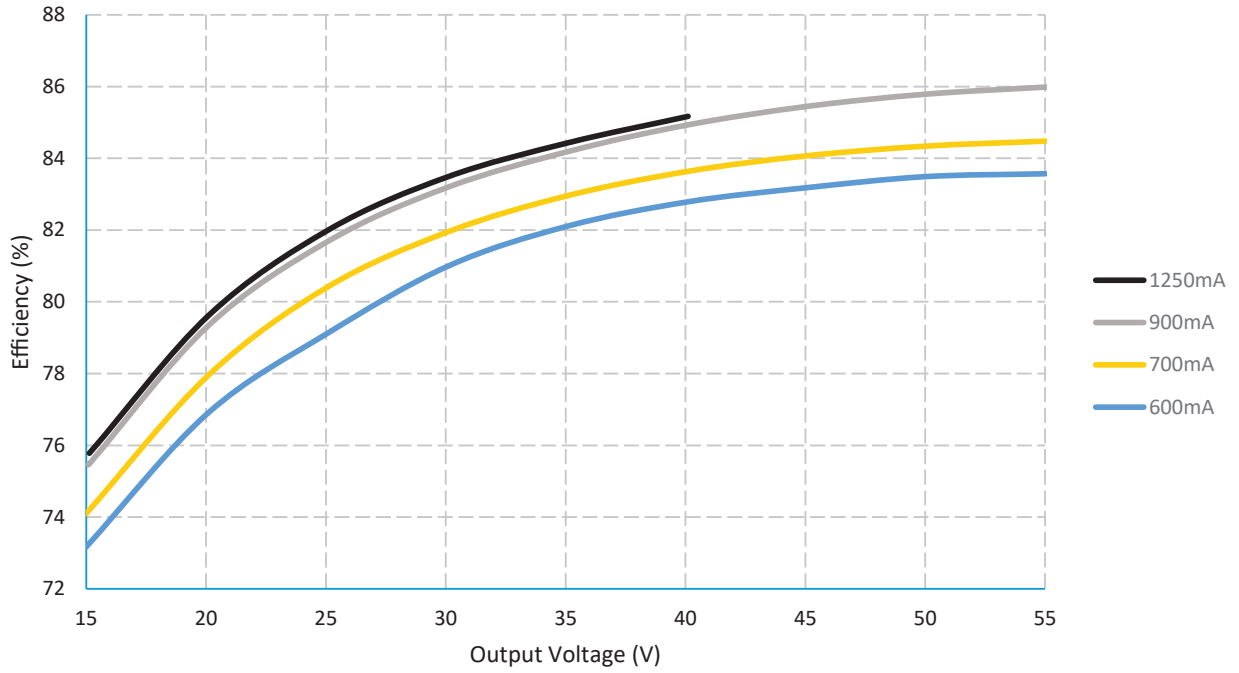
Efficiency @120V
