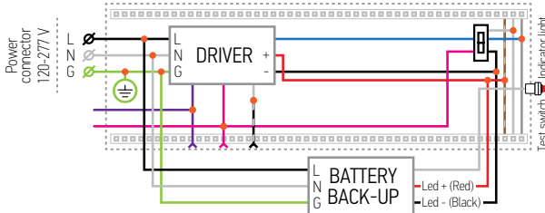
WHB5B-NEOX with battery back-up kit (100-320W)
