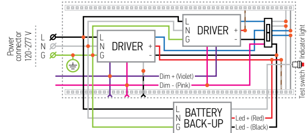
WHB5B-NEOX with battery back-up kit (500W)
