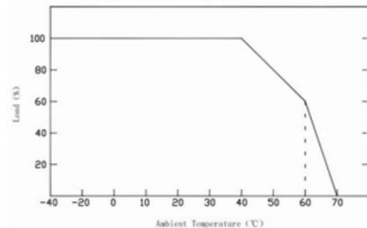
Derating Curve
