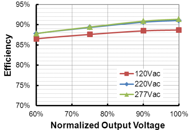
EUD-150S210DTL (I o =2100mA) Efficiency vs. Output Voltage
