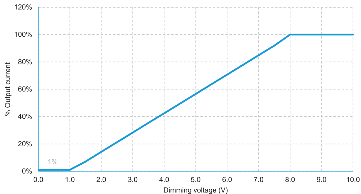
0-10V Dimming
