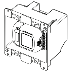
Inside a 2-gang J-box
