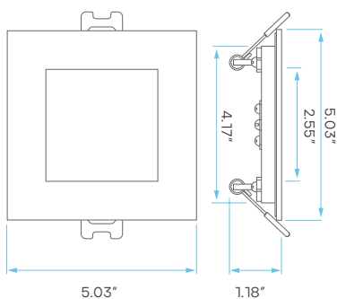
CUTOUT: Ø 4.25"
