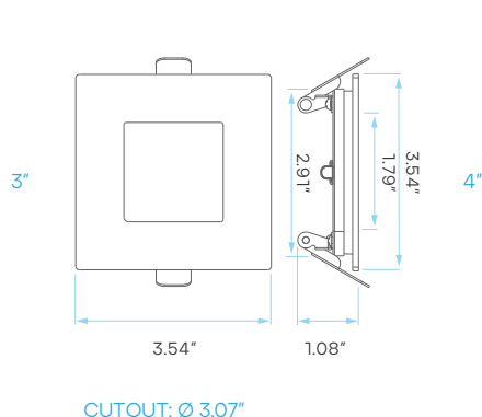
CUTOUT: Ø 3.07"
