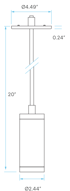
ASSEMBLED VIEW
