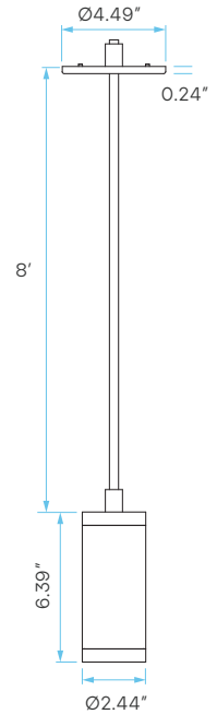
ASSEMBLED VIEW
