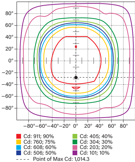
ISOCANDELA PLOT
