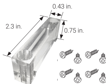
Acrylic Standoff - Pack of 4 - 0.75 in.
