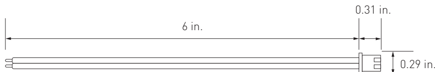
Hardwire Power Cable - 6 in.
