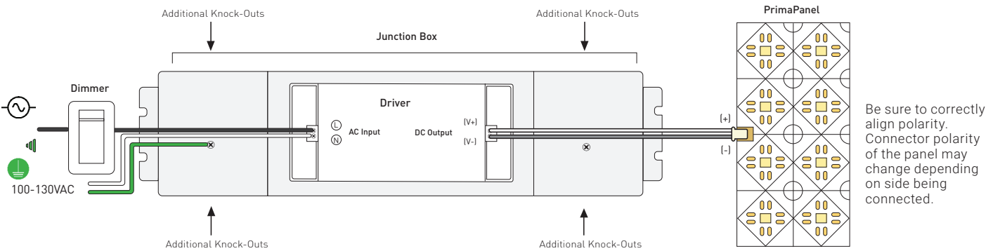
White model for 60W and lower
