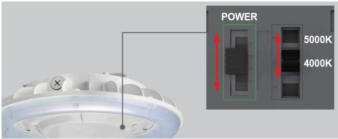
CCT Color and Lumen/Wattage Selectable Switches
