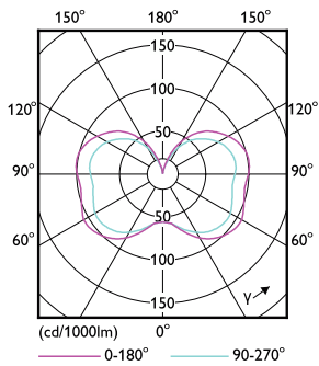
Light Distribution Diagram - 54-45-36CC/LED/3PW/3CCT/Ex39 BB 3/1
