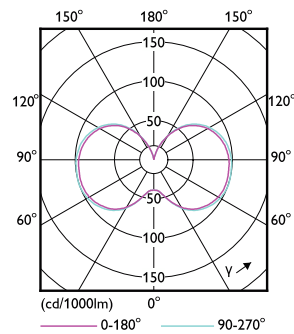
Light Distribution Diagram - 115CC/LED/850/LS EX39 G2 BB 277-480V 3/1
