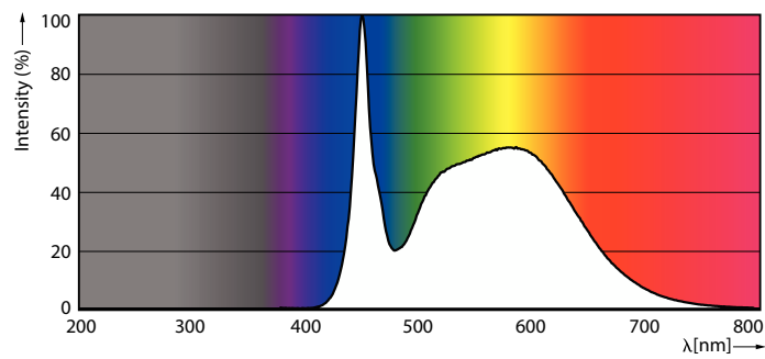
Spectral Power Distribution Colour - 115CC/LED/850/LS EX39 G2 BB 277-480V 3/1
