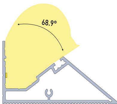
Surfa KnifeEdge 4 in. Beam Angle
