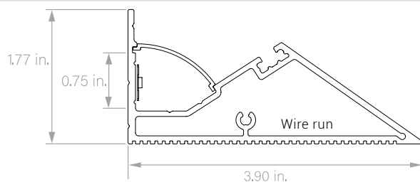
Surfa KnifeEdge 4 in. Channel
