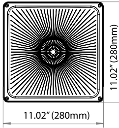
100W CANOPY
