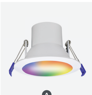
Spektrum+ 4" Round Regressed Downlight 120V AC, 9W, 348Lm SPKPL-RDLRE4R-RGBTW-WH
