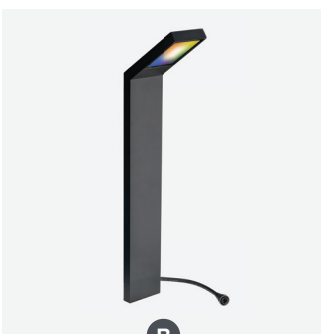
B Pathway Light 12V AC/DC, 600Lm/fixture, 9W/fixture SPKPL-PTWY-RGBTW-BK
