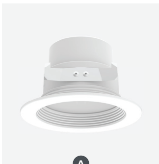
Spektrum+ 4" RGB+TW Downlight 120V AC, 800Lm, 10.5W/module SPKPL-DL4B-RGBTW-WH
