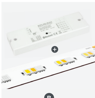
RGB+TW Tape Light 24V DC, 410Lm/ft, 7W/ft SPTL-RGBTW With Receiver (SPKPL-REC-TB-5CH)
