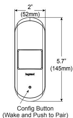
With Plate Mount Attached
