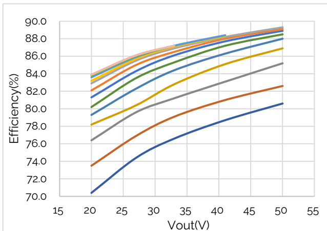
Figure 8: Efficiency @ 347VAC
