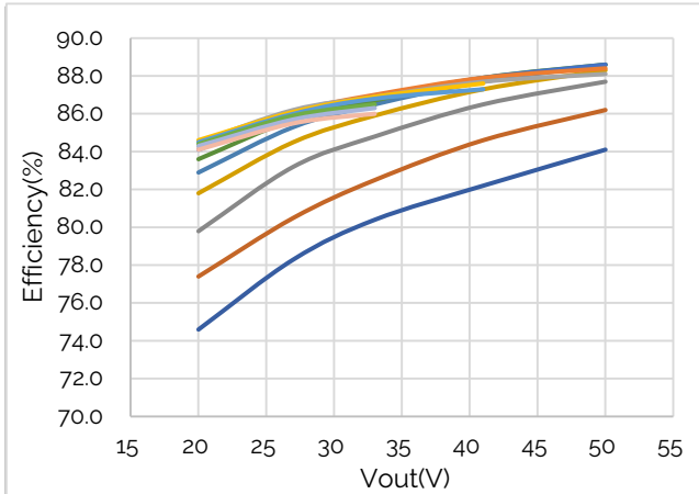
Figure 6: Efficiency @ 120VAC
