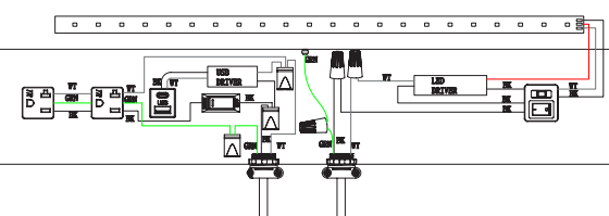
120V AC for Light 120V AC for Receptacle(s) Separate Circuits
