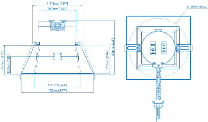
DRS 4S LS12 G4 FSK - 4" Square
