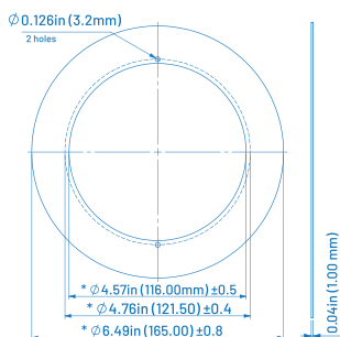
DT GR 4R W - 4" Round Goof Ring
