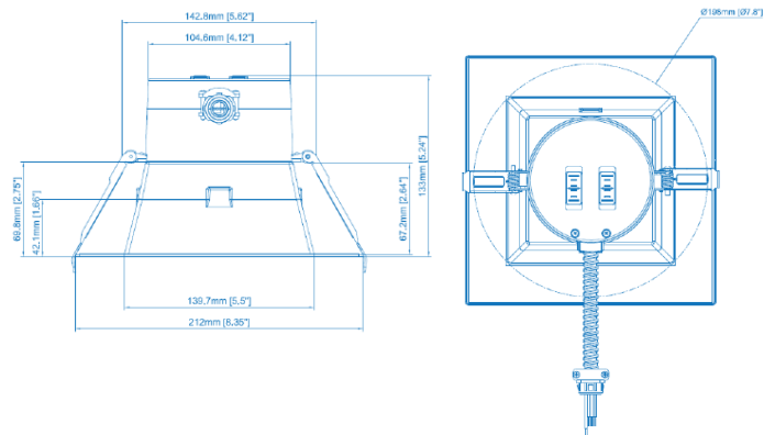
DRS 6S LS15 G4 FSK - 6" Square
