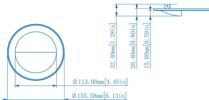
DRS 4R W G3 - Wall Wash for 4" Round Downlights
