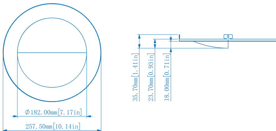
DRS 8R W G3 - Wall Wash for 8" Round Downlights
