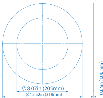
DT GR 8R W - 8" Round Goof Ring
