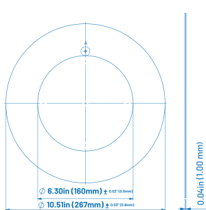
DT GR 6R W - 6" Round Goof Ring
