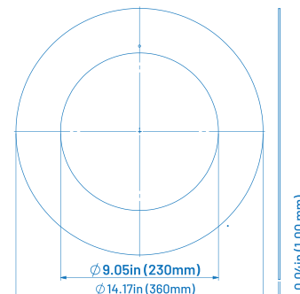
DT GR 10R W - 10" Round Goof Ring
