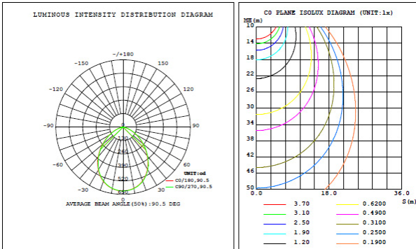
DRS 8R LS34 G4 9FSK - @25W, 5000K CCT
