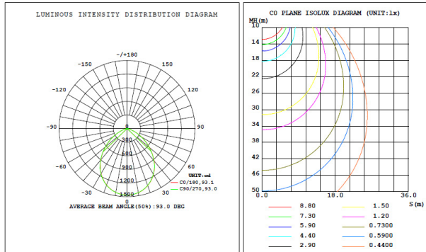
DRS 10R LS42 G4 9FSK - @36W, 5000K CCT
