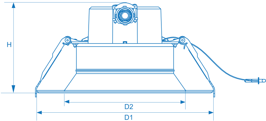
DRS G4 - Retrofit Commercial Downlight - Round
