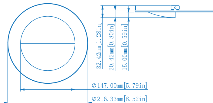
DRS 6R W G3 - Wall Wash for 6" Round Downlights
