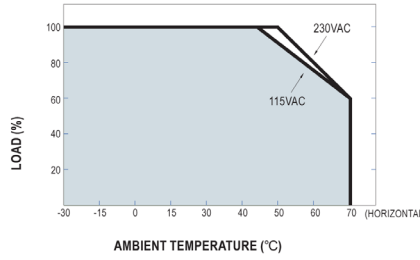
■ Derating Curve
