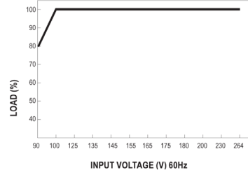
■ Static Characteristics
