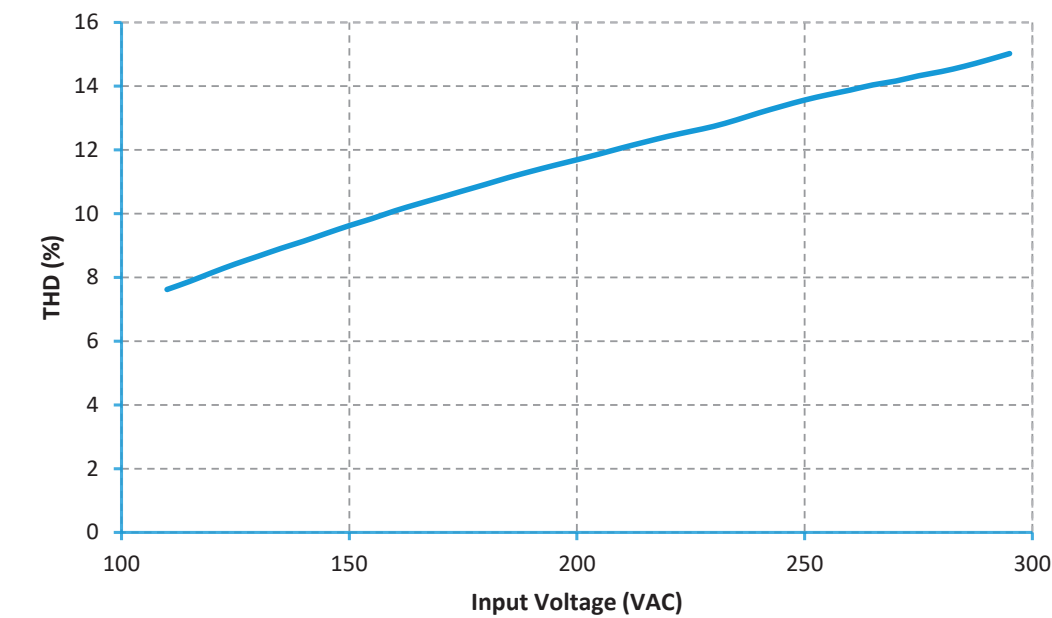
THD vs. Input Voltage (Full Load)
