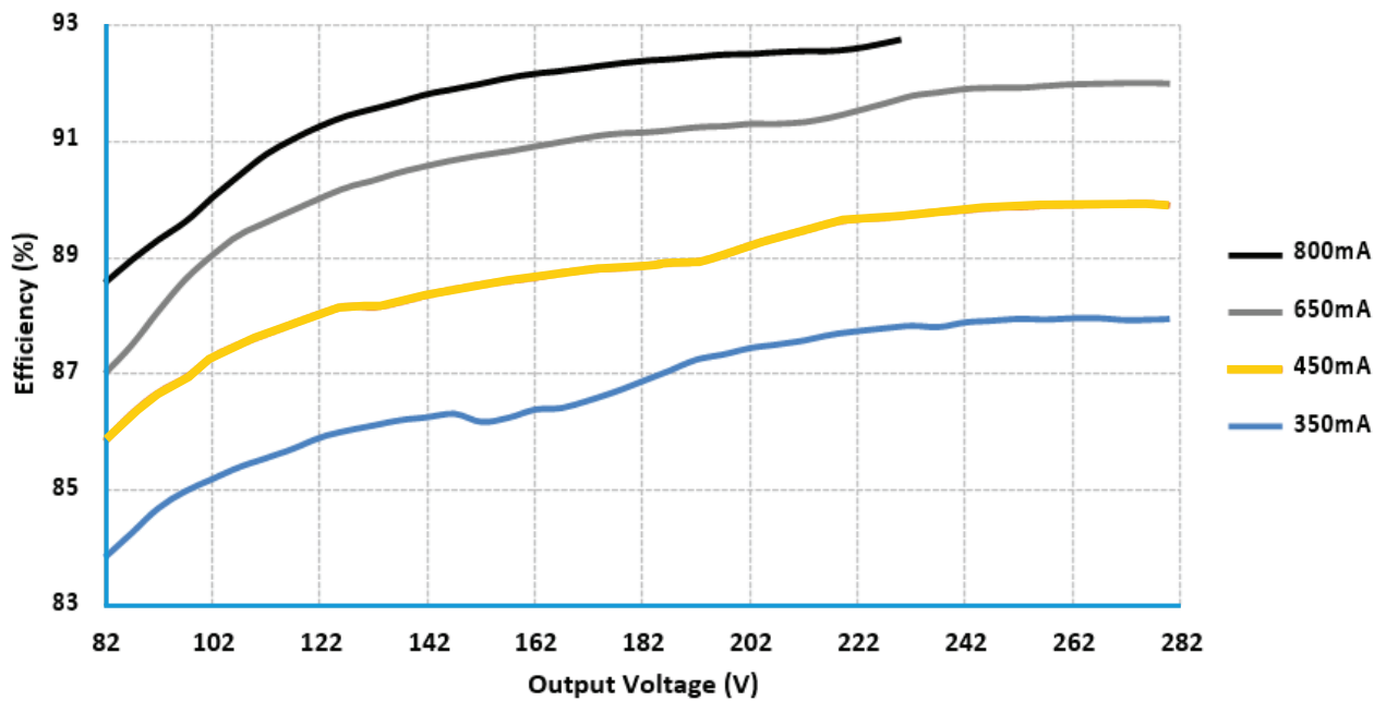
Efficiency @ 277V
