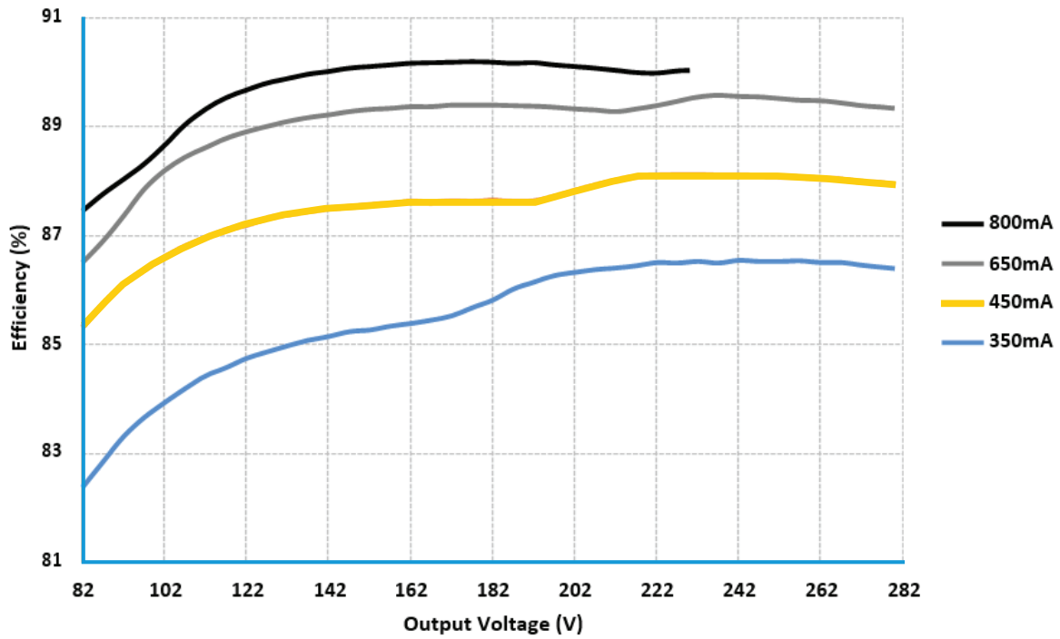
Efficiency @ 120V
