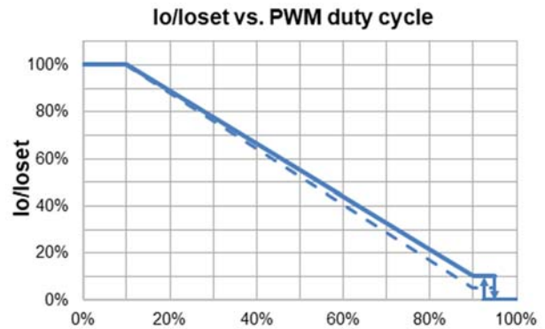
Implementation 4: Negative logic PWM duty cycle
