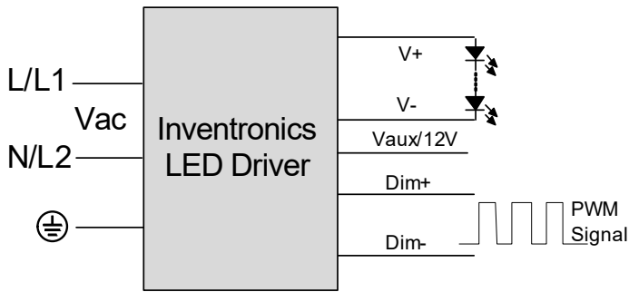
Implementation 4: Negative logic PWM duty cycle
