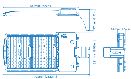
ALF LS450/LS600 W/ Adjustable Pole Mount
