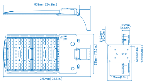
ALF LS450/LS600 W/ Trunnion Mount
