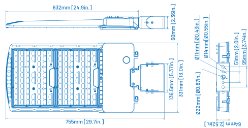
ALF LS450/LS600 W/ Trunnion Mount
